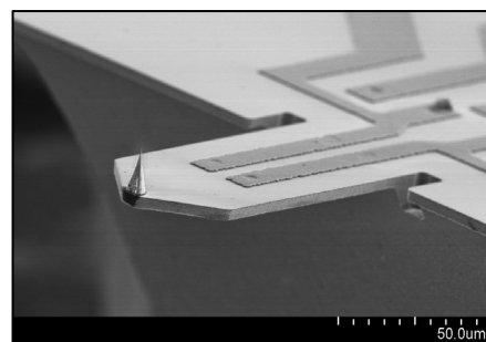
PRS-L100-F400-SCD cantilever with Al tracks for reading out the sensor signal
