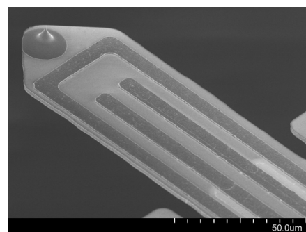
Tip side of a PRSA-L100 cantilever with Al tracks for reading out the deflection signal
